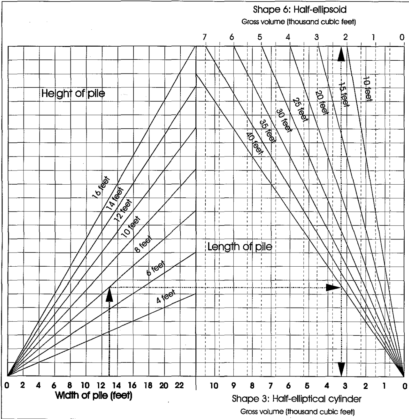
Figure 5—The nomagram assists in determining gross pile volumes (X-axes at upper and lower right) for shape codes 6 and 3, respectively, by width (X-axis at lower left), height (diagonal lines at left), and length (diagonal lines at right).
