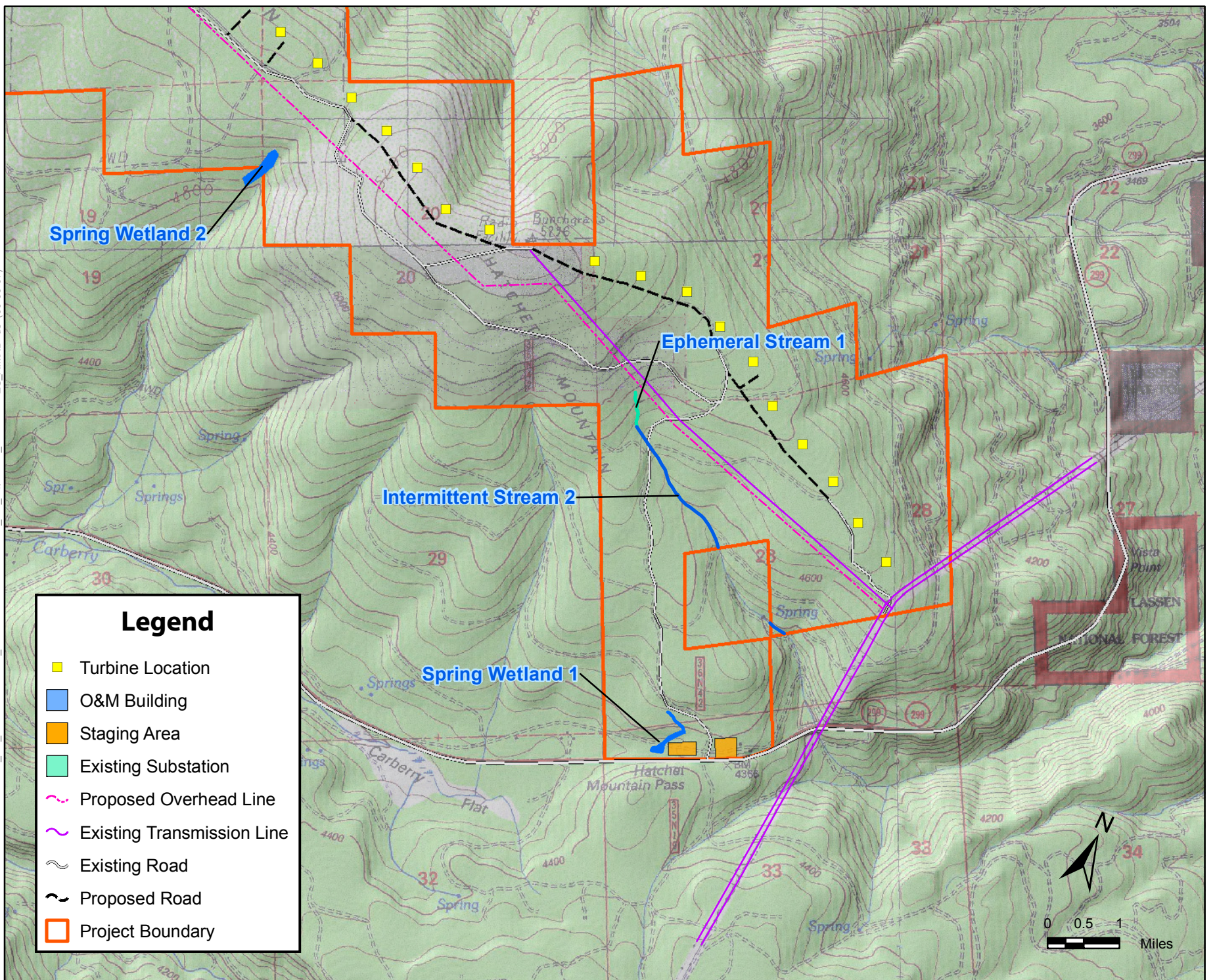
Figure 3.4-2 Aquatic Resources in the Hatched Ridge Wind Project Area
