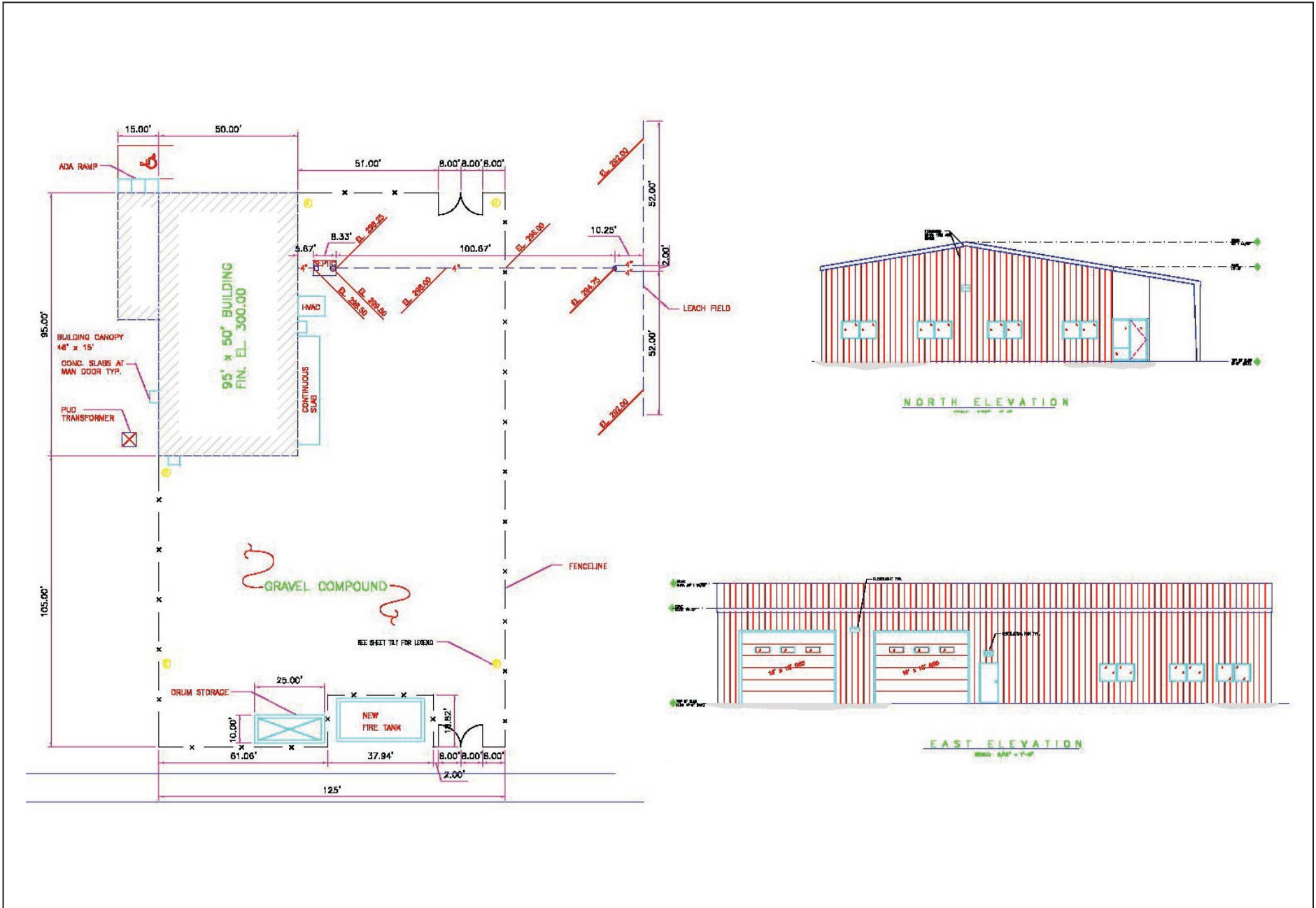
Figure 2-5 Typical Operations and Maintenance Building
