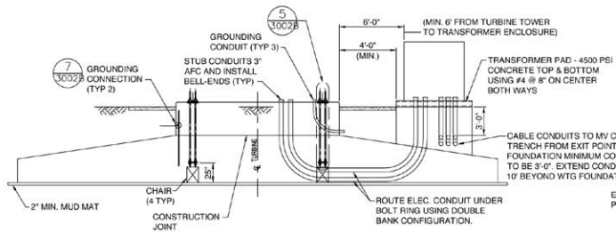
A-A SECTION: TRANSFORMER AND CONDUIT ROUTING SCALE: 3/16" = 1'-0"
