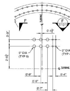
4 DETAIL: PEDESTAL CONDUIT LOCATION SCALE: 1/2\"/>
