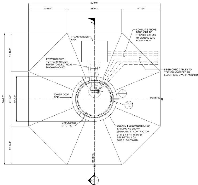
1 PLAN: TURBINE FOUNDATION SCALE: 3/16" = 1'-0"
