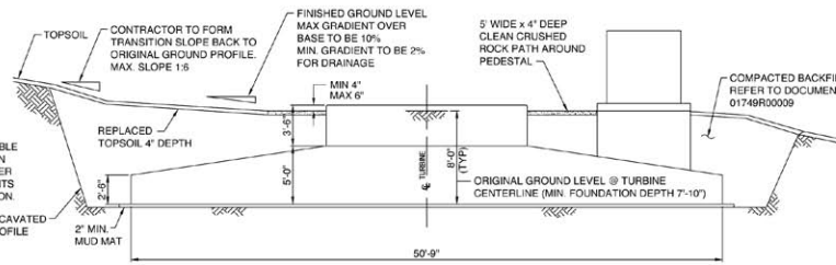
A-A SECTION: FOUNDATION GRADING SCALE: 3/16" = 1'-0"
