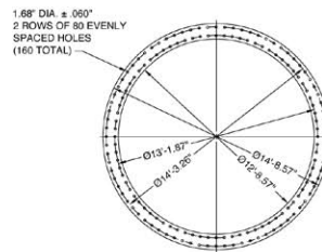
2 DETAIL: EMBEDMENT RING SCALE: 1:4
