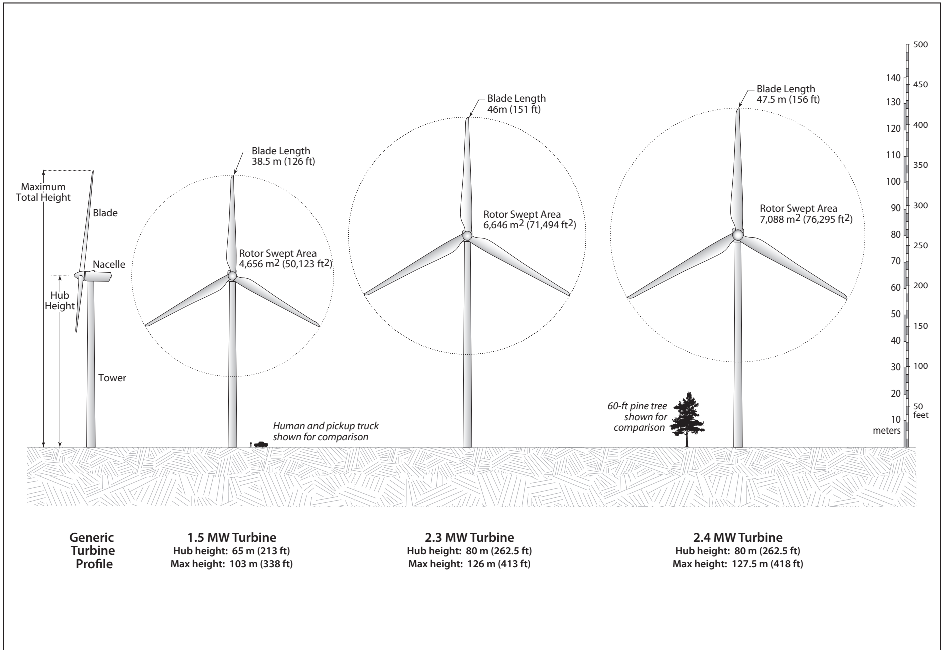
Figure 2-3 Turbine Options for the Hatchet Ridge Wind Project
